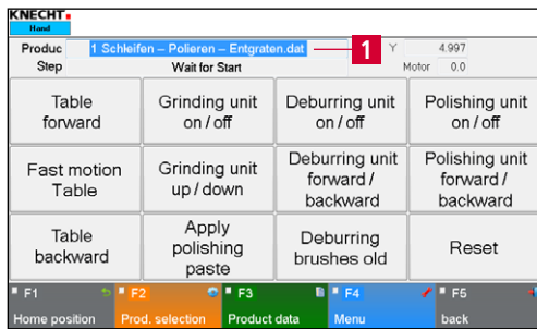
Figure 8-5 Main screen
