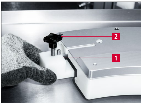
Figure 7-4 Mounting the limit switch cam
