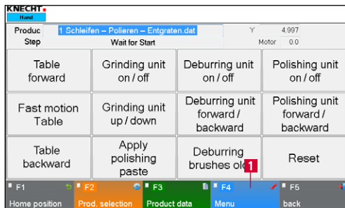
Figure 8-31 Main screen
